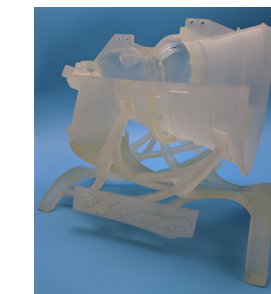
3D printed receiver for refueling at sea
