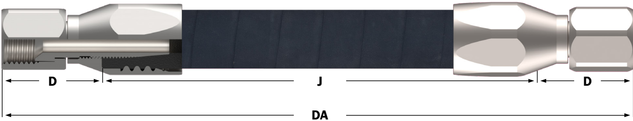
To determine "J" length (length of hose), deduct "D" dimensions of both end fittings from "DA" (overall length)
